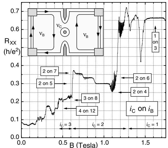
FIG. 2. Four-terminal R_{xx} vs B in the integer QH regime; horizontal arrows (labeled i_C on i_B ) show quantized values of R_L . The negative bias on the front gates depletes the antidot-constriction region so that \nu_C is smaller than \nu_B in the bulk. The inset illustrates the case \nu_C \approx 1 on \nu_B \approx 2 .
