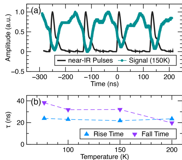
FIG. 4. (a) Transient response to a 7.8 MHz pulse train in the near-IR with 1400 nm \leq \lambda \leq 2400 nm at T = 150 K and V = -1 V. (b) Rise and fall times of the readout circuit to the 7.8 MHz near-IR pulse train at V = -1 V reverse bias as a function of T in the 77 – 200 K range.
