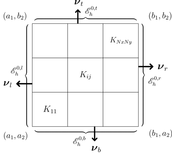
Figure 1: The 2D mesh \Omega_h
